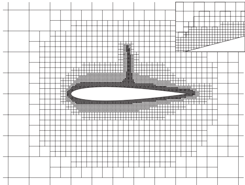
Figure 11.9 Block-structured mesh for a transonic aerofoil. Inset shows cut cells near aerofoil surface. Also note additional grid refinement in the flow region to capture a shock above the aerofoil
