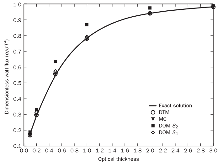
Figure 13.11 Comparison of numerical results for one-dimensional temperature prescribed problem
