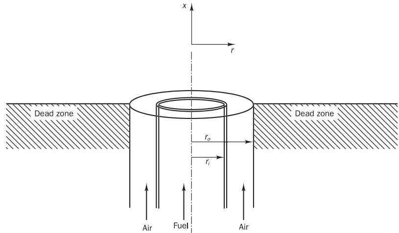
Figure 12.3 Schematic of the problem considered
